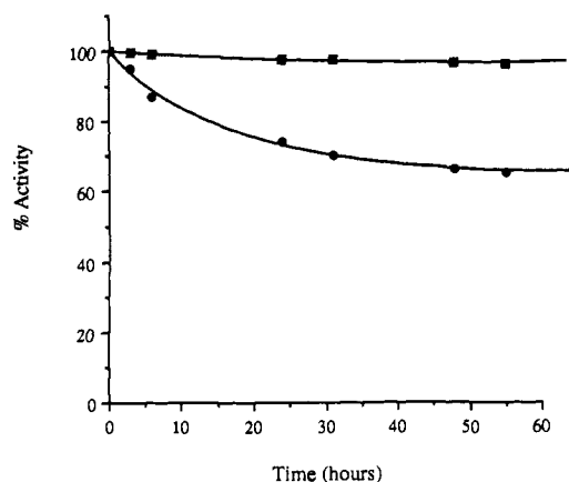
Figure 2. Stability study of both the native (■) and the tagged (●) CMP-sialic acid synthetase.
