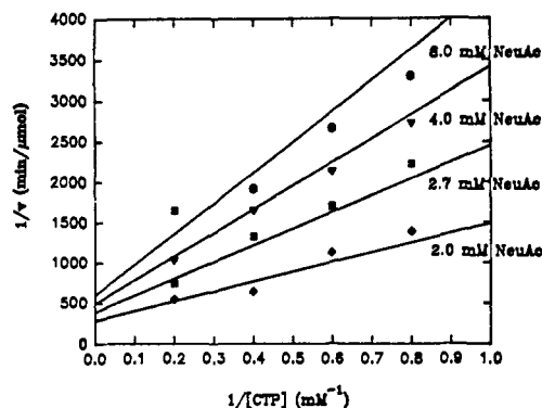
Figure 4. Lineweaver-Burk plot of tagged CMP-sialic acid synthetase for the determination of kinetic parameters. The initial rates at different substrate concentration were accumulated to fit in the equation v = V[A][B]/([A][B] + K_a[B] + K_b[A] + K_aK_b) , where K_a and K_b represent the Michaelis constants for CTP and NeuAc and are 1.99 and 4.8 mM, respectively. K_i is the dissociation constant (or inhibition constant) for CTP and is 1.97 mM.
