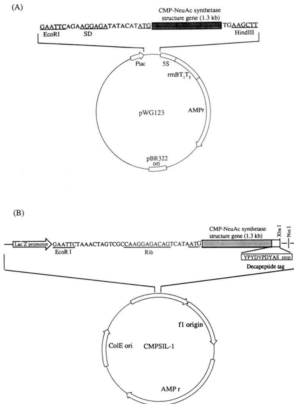
Figure 1. Plasmids pWG123 and CMPSIL-1 for overexpression of the native and tagged CMP-NeuAc synthetase.
