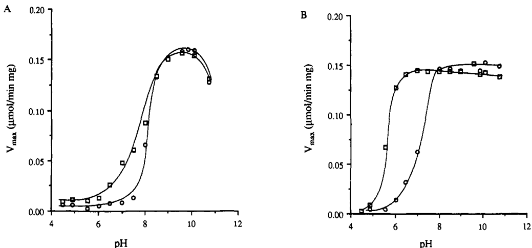
Figure 3. (A) pH profile of the tagged CMP-sialic acid synthetase. (B) pH profile of native CMP-sialic acid synthetase: (O) in the presence of 6 mM \text{MnCl}_2 ; (□) in the presence of 20 mM \text{MgCl}_2 . The buffers were prepared in 50 mM Na cacodylate and 0.2 mM DTT, from pH 4.5 to 7.5, and in 0.2 M Tris and 0.2 mM DTT, from pH 8 to 10.8.
